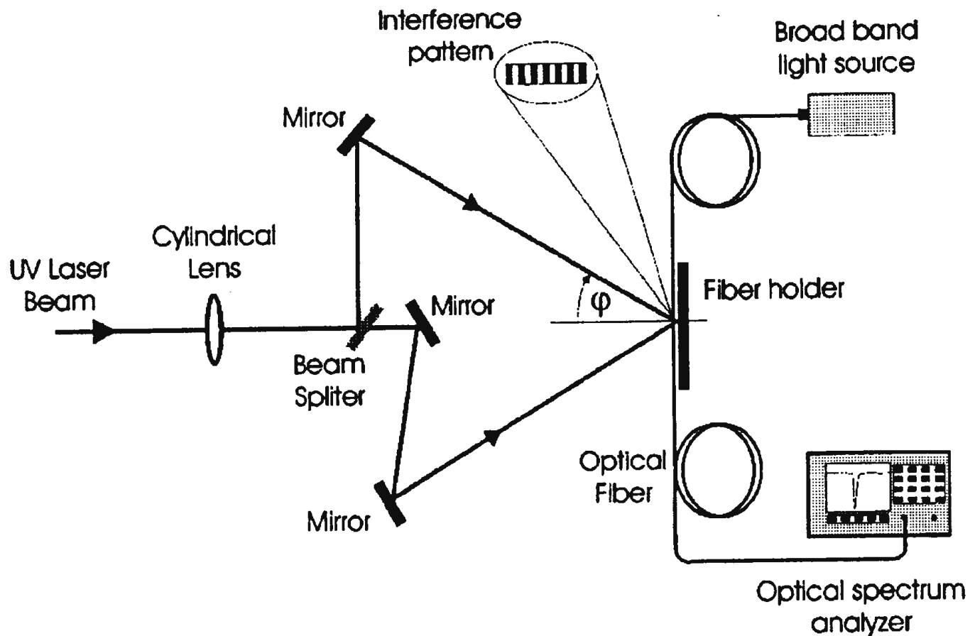
Experimental setup for the production of Bragg gratings in optical fiber by UV irradiation interferometer method.
